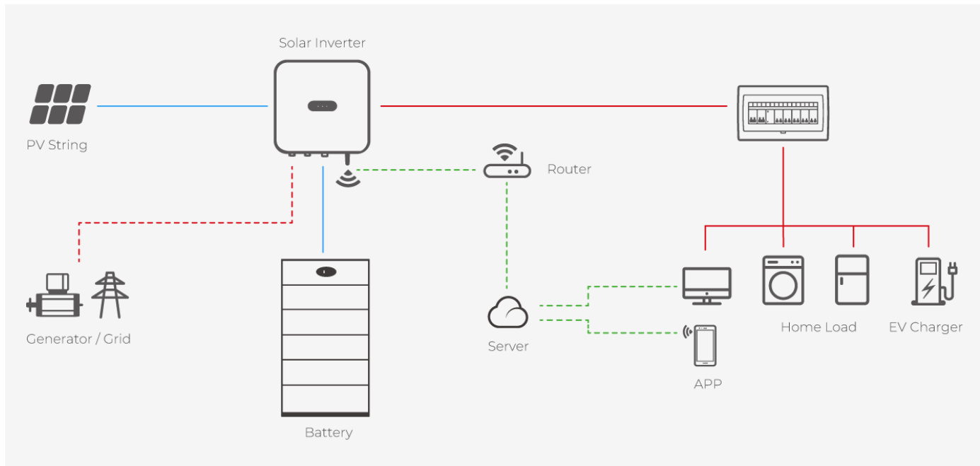
Figure 1 blockIQ Layout
